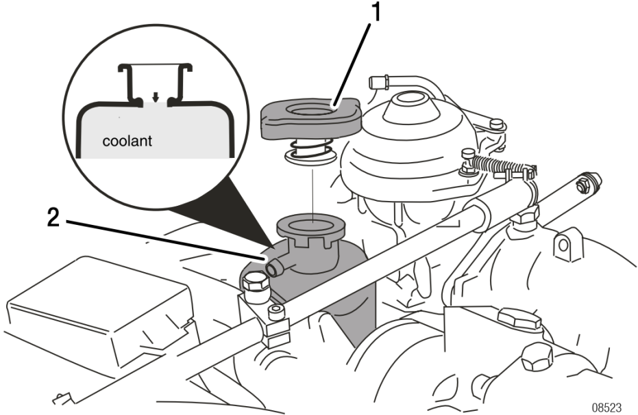
Figure .1: Expansion tank
